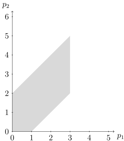
(a) The set of Walrasian price vectors.
