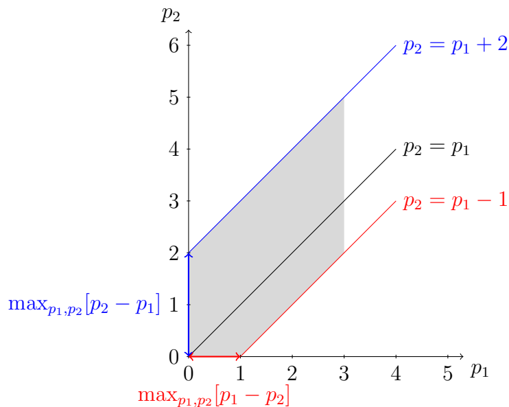
(b) The largest net Walrasian prices.
